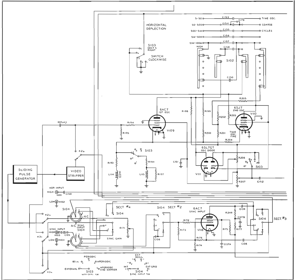
FIG. 2. Circuit diagram showing how the Sliding Pulse Generator and Video Stripper were connected to 715-B Scope Circuits.
