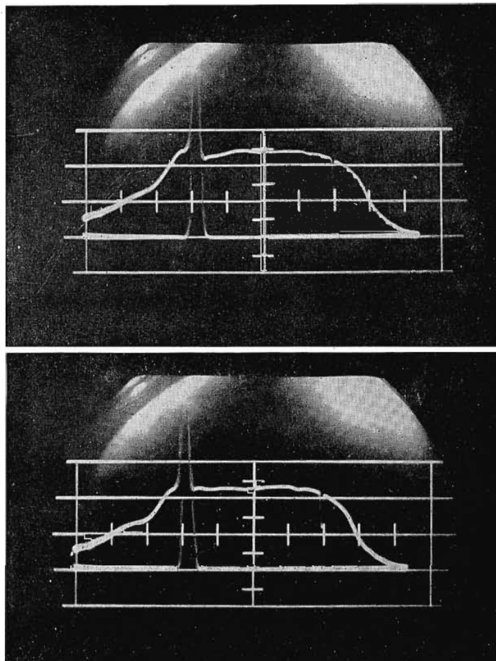
FIG. 8. Upper and lower sideband inequality shown before and after proper neutralization using the BW-5A.
