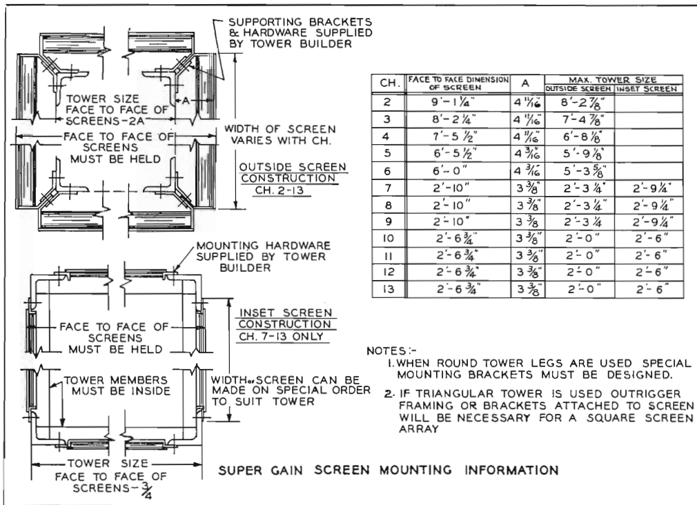
FIG. 9. Face-to-face dimensions of supergain antenna screens.
