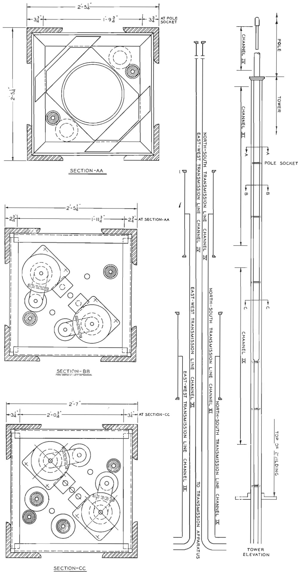
FIG. 6. Sketch showing transmission line runs, conduit requirements, and location for the core of the "multiple-use" Foster antenna structure.
