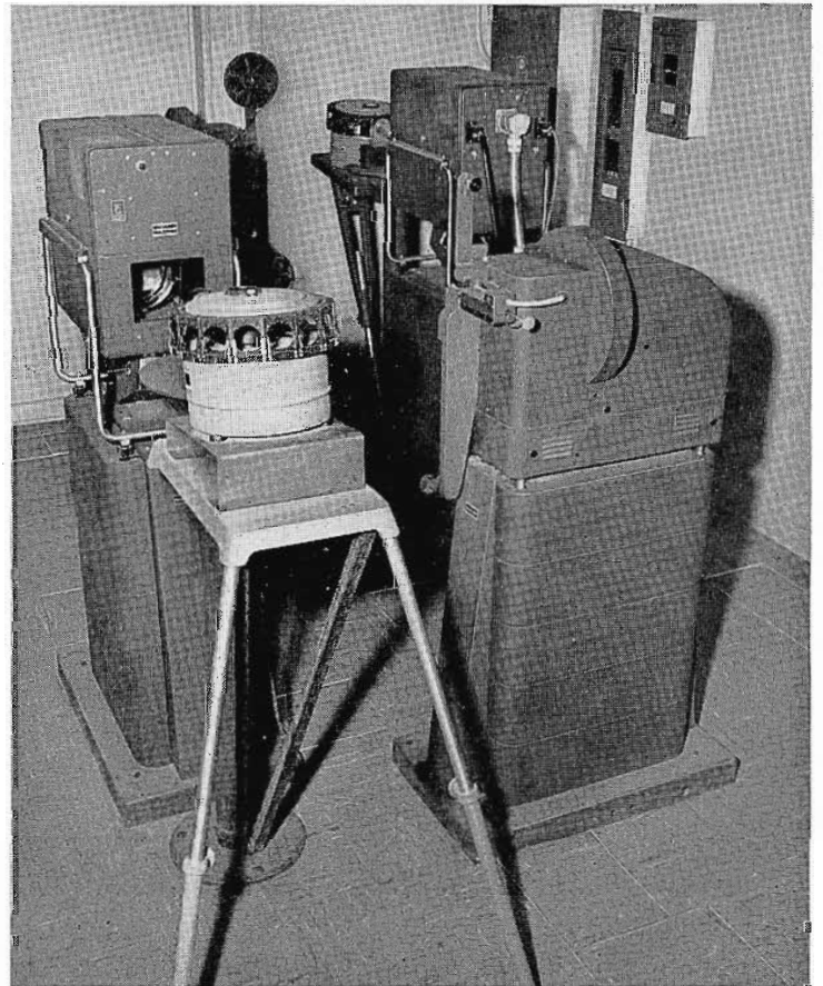
FIG. 14. Film room equipment consists of two RCA TK-20C film camera chains, two TP-2A Automatic Slide Projectors and two TP-9C Multiplexers.
