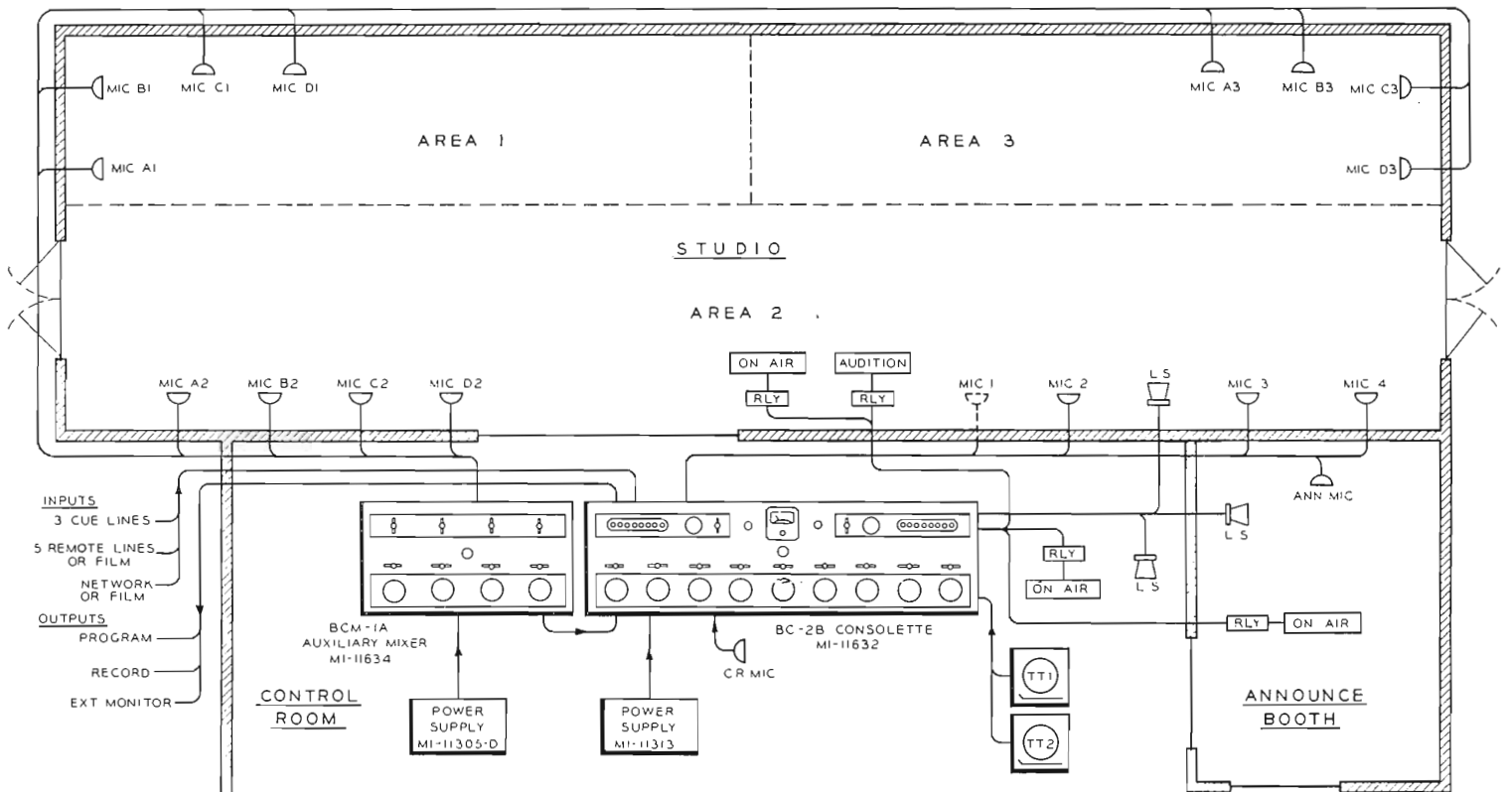
FIG. 6. Diagram showing a typical layout of the BCM-1A Auxiliary Mixer and BC-2B Studio Console.
