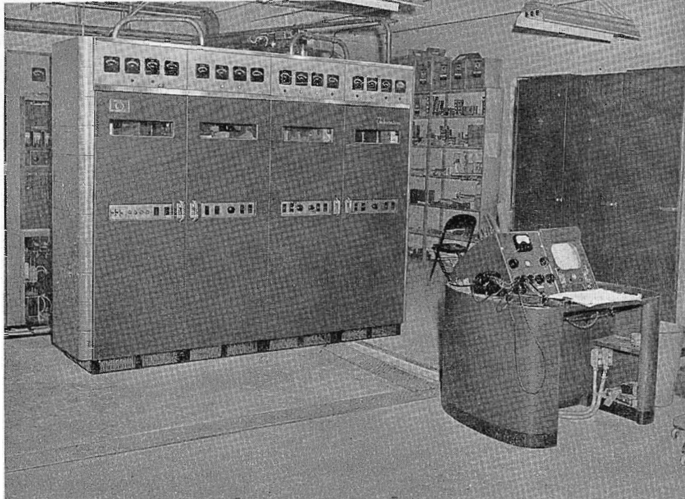
FIG. 6. Shown here is the RCA TT-2AL interim transmitter and control console. Directly behind the 2-KW unit is the TT-10AL ready for the change to higher power.
