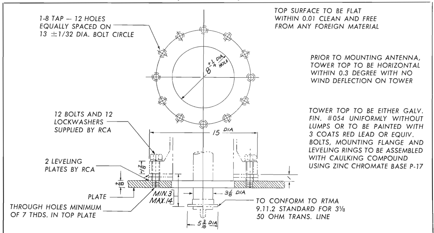
FIG. 10. Tower top installation drawing for 8 1/4" UHF antenna.
