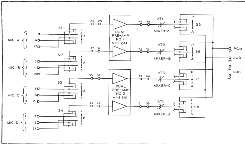
FIG. 3. Block diagram of the BCM-1A which permits the use of any of four of 12 additional microphone inputs.
