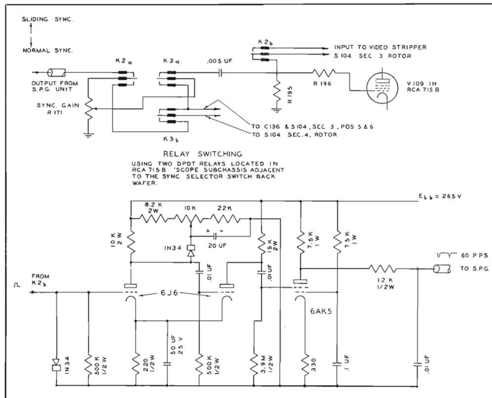
FIG. 1. Schematic diagram of the KING-TV Relay Switching and Video Stripper used for 715-B "Scope" modification.
