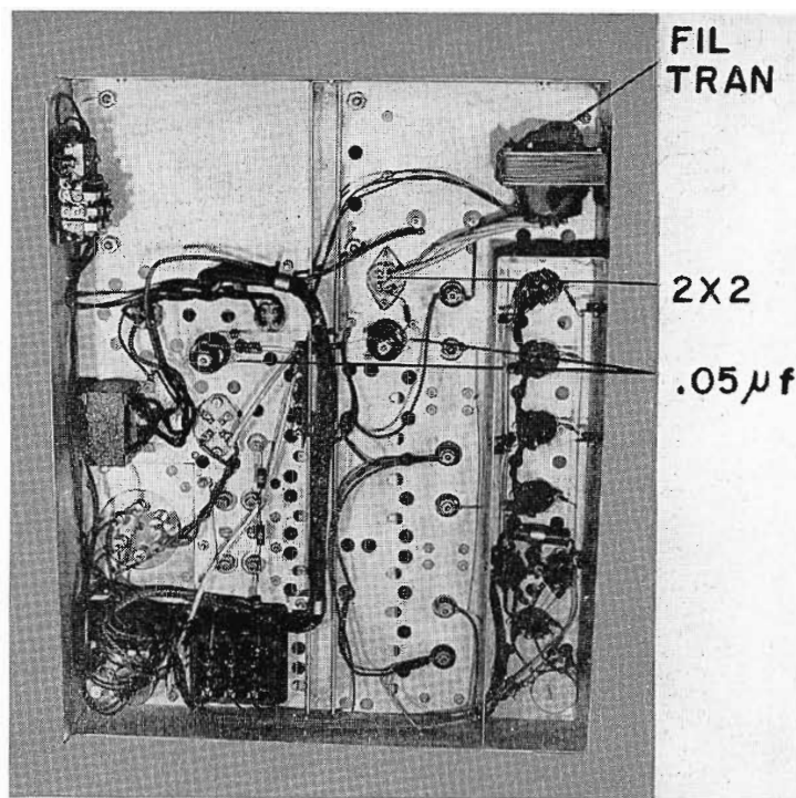
FIG. 5. Bottom view of modified 715-B Power Supply.
