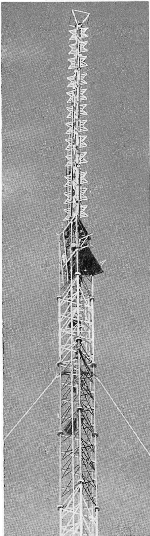
FIG. 5. The completed antenna installation is shown here on its triangular, 500-foot guyed tower. It was erected through the combined efforts of the KTBC engineering staff, RCA engineering, Ideco and the Seago Construction Co., erectors.
