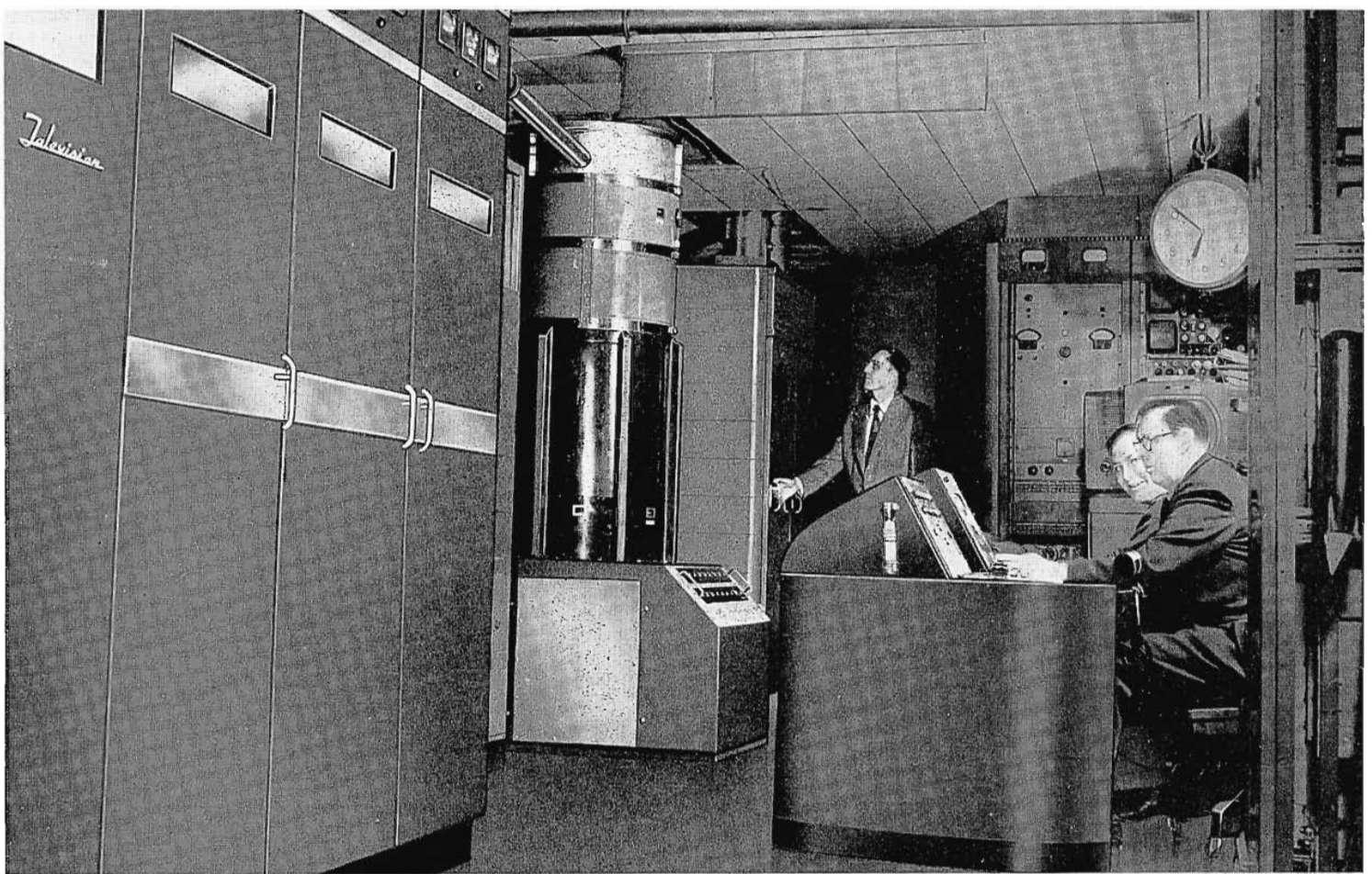
FIG. 7. View of the TT-25AL high-power amplifier and TT-5A driver unit. Jerry King-Ellison is shown at the power amplifier cabinet and Clyde Green and Ray Johnson at the transmitter console.
