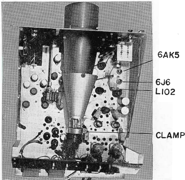
FIG. 6. Top view of the main "Scope" chassis showing the 5CPI as now mounted in the chassis. Note that new "C" clamp is installed.
