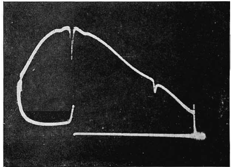
FIG. 5. Another response obtained by the diode method when the lower sideband is partially cut off.
