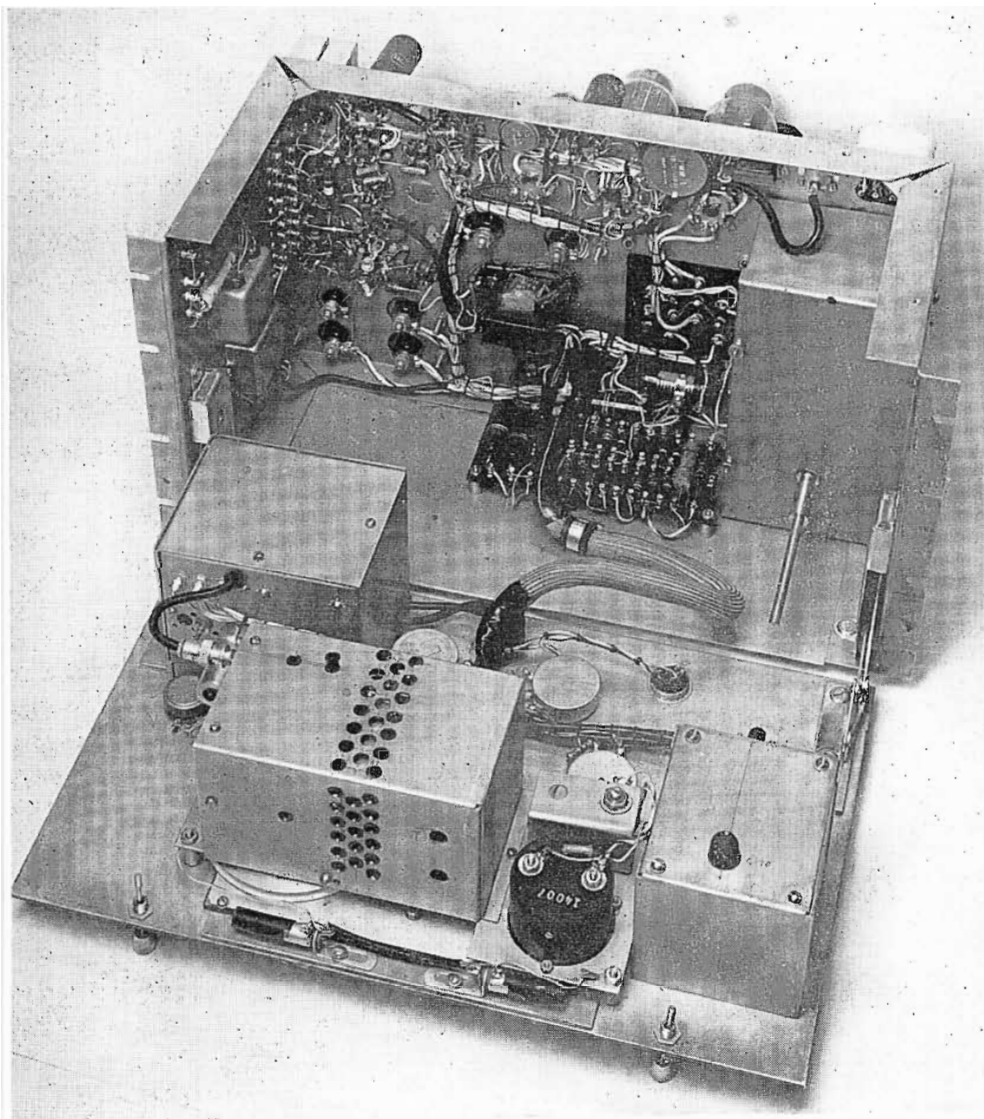
FIG. 14. View with door open and cover removed.
