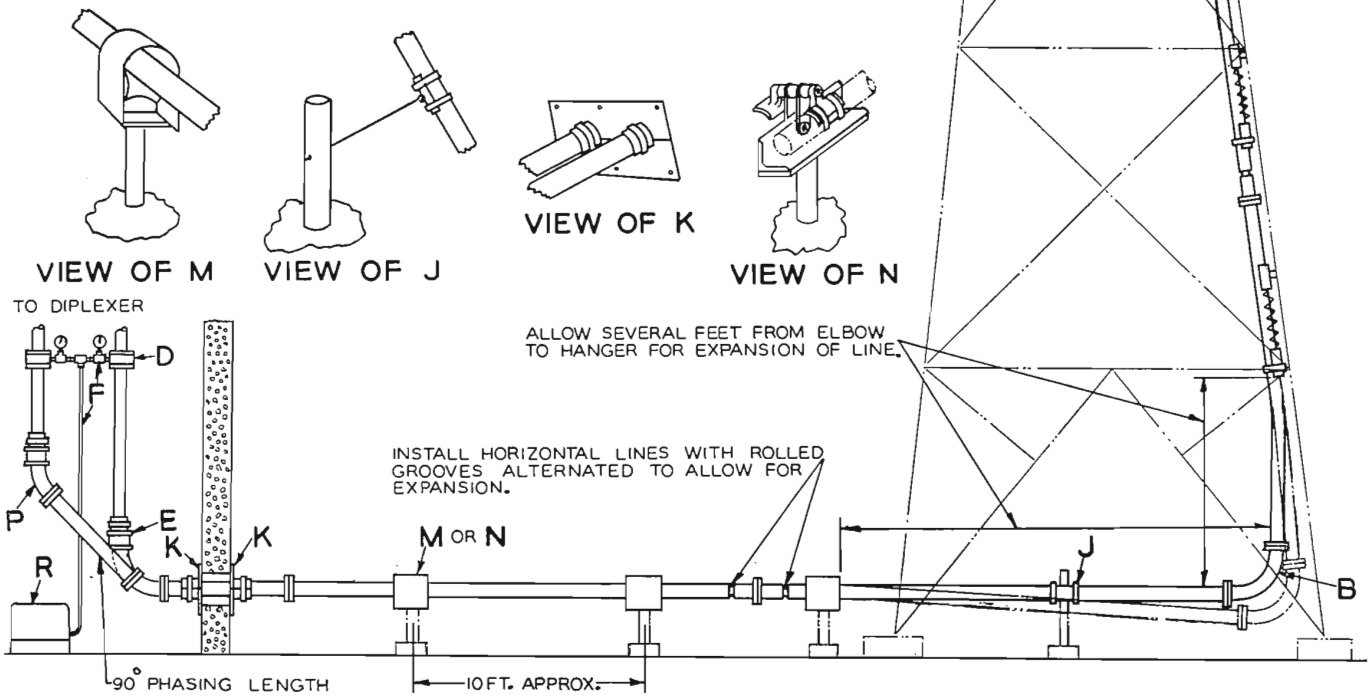
FIG. 11. Typical installation of VHF transmission line run on tower.
